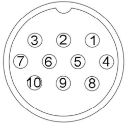
Plug viewed from solder side
